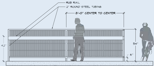
Railing Option 4
