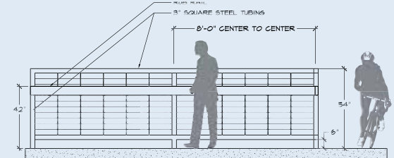
Railing Option 3
