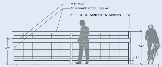
Railing Option 12
