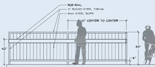
Railing Option 5
