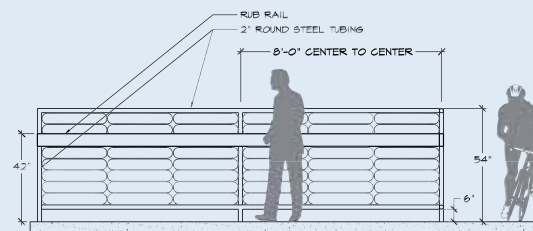
Railing Option 11
