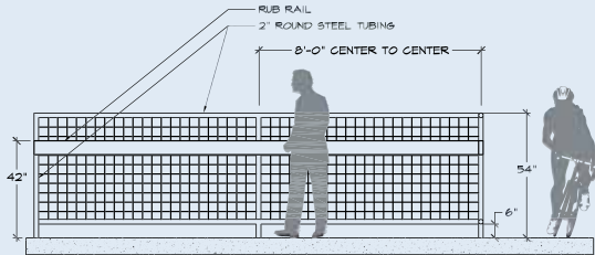
Railing Option 7
