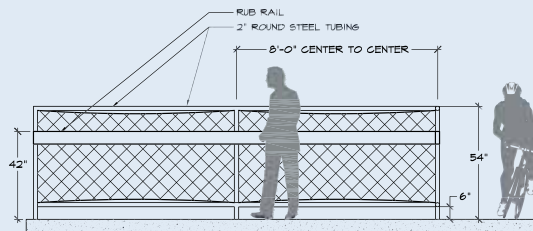
Railing Option 8
