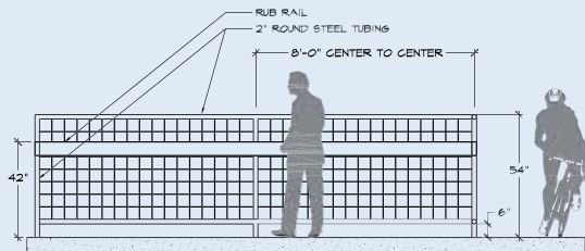
Railing Option 10
