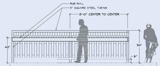
Railing Option 9
