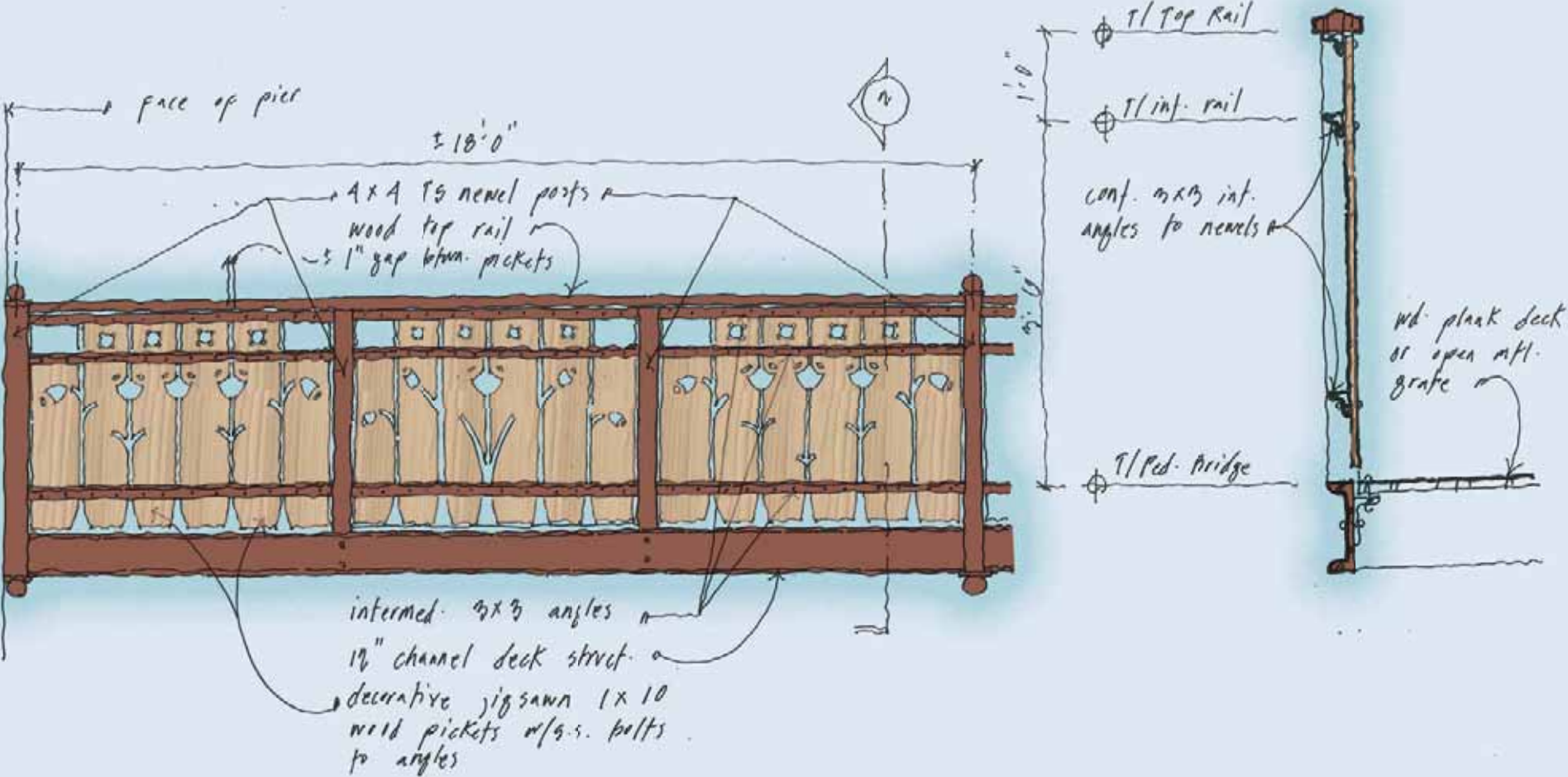
1. Decorative Railing Elevation
