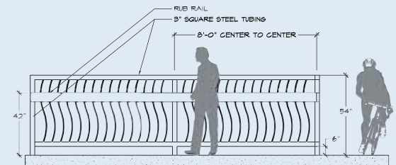
Railing Option 6
