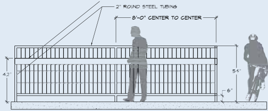
Railing Option 1
